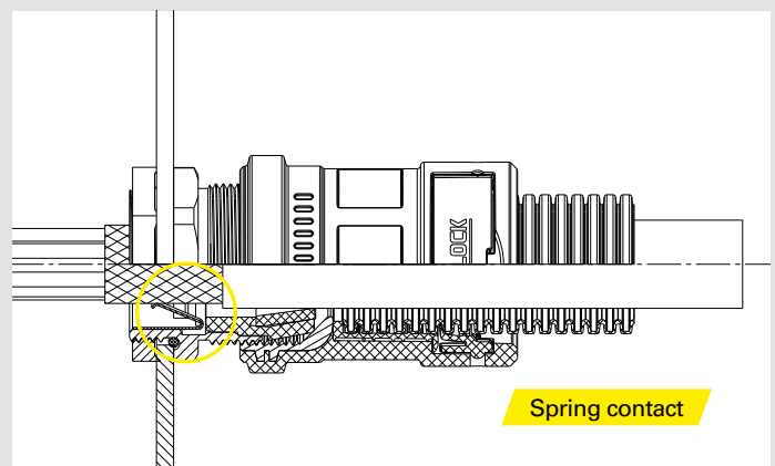
FIPSHIELD® with EMC Spring
