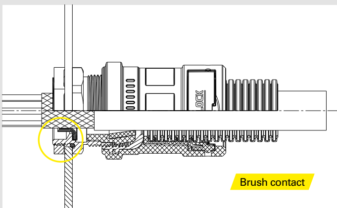
FIPSHIELD® with EMC Brush
